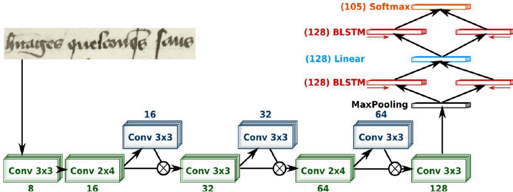
Fig. 1. Neural network architecture.
